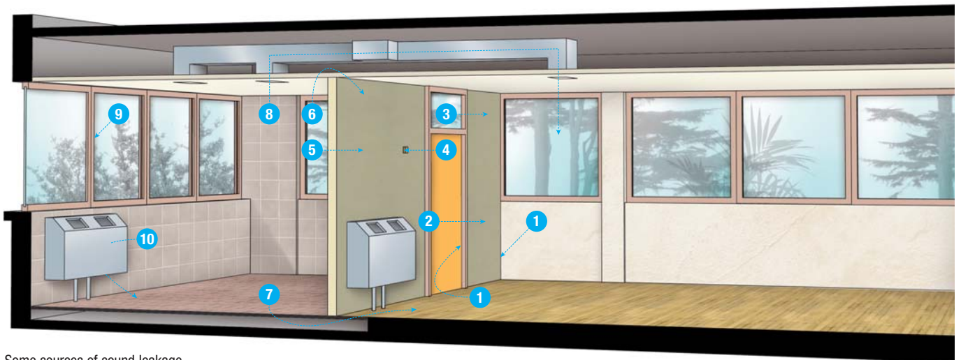
Some sources of sound leakage
